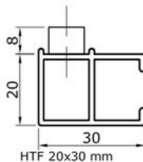
HTF geleider 20 x 30 mm
